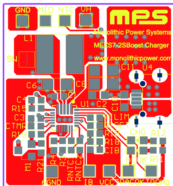
Figure 4: Top Layer
