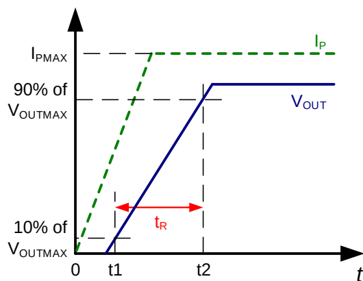
Figure 6: Rising Time ( t_R )
