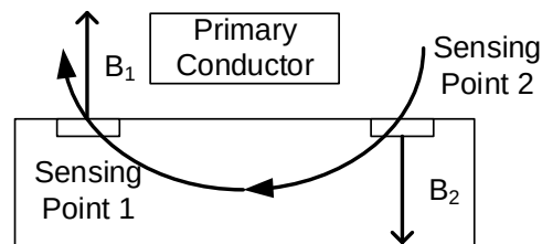
Figure 3: Sensor's Cross-Section
