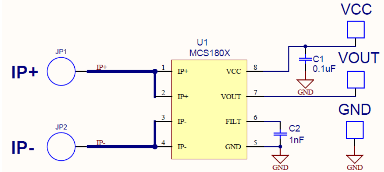
Figure 11: Application Circuit
