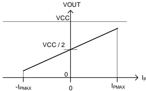
Figure 2 : sensor output function
