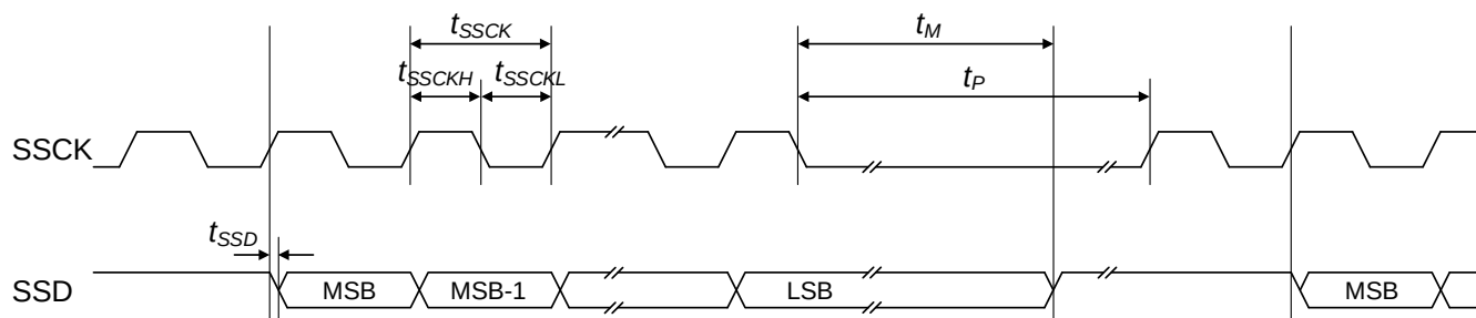
Figure 15: SSI Timing
