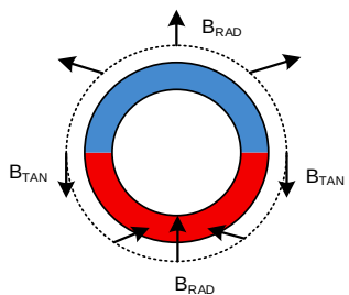
Figure 28: Side-Shift Field
