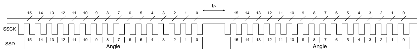
Figure 24: Two Consecutive 16-Bit SSI Angle Readings (with Required Dead Time Between the Frames)
