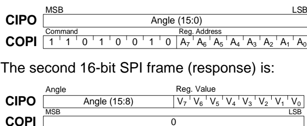
Figure 13: 32-Bit Frame Read Multi-Turn/Speed Operation
