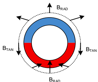
Figure 28: Side-Shaft Field
