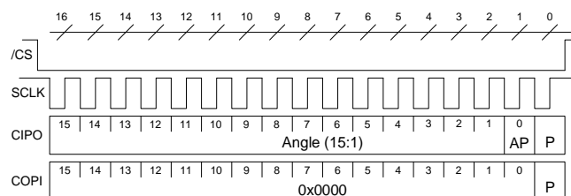
Figure 21: Angle Output with Parity Bit when PRT = 1 and APRT = 1
