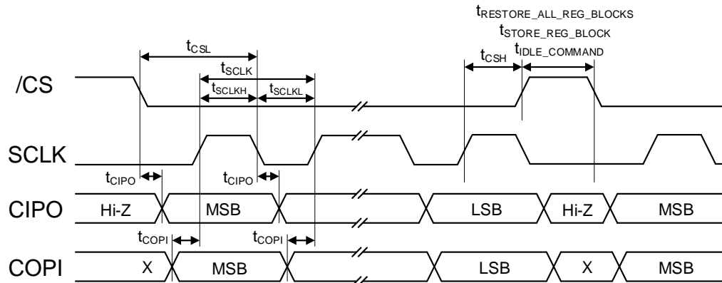
SPI Mode 0
