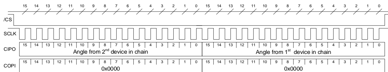
Figure 46: SPI Read Angle for Two DaisyChained MA600 Devices
