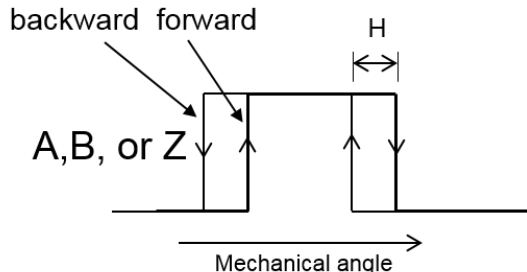
Figure 24: Hysteresis of the Incremental Output
