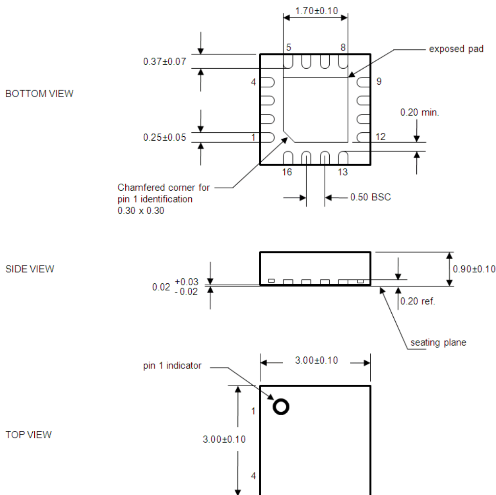
QFN-16 (3mmx3mm)
