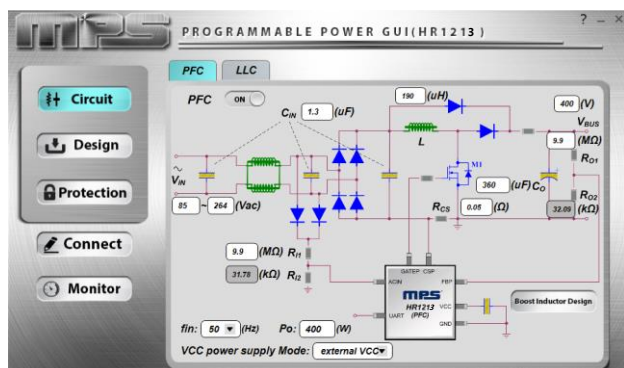
Figure 5: HR1213 GUI
