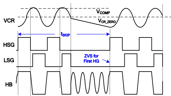
Figure 31: LLC Skip Mode Operation
