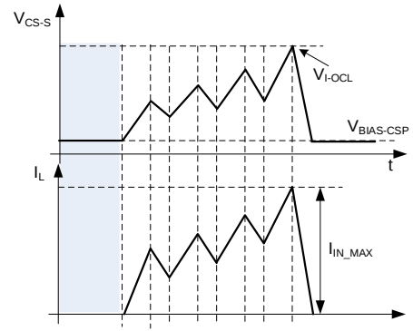
Figure 18: V_{CS\_S} Voltage Waveforms
