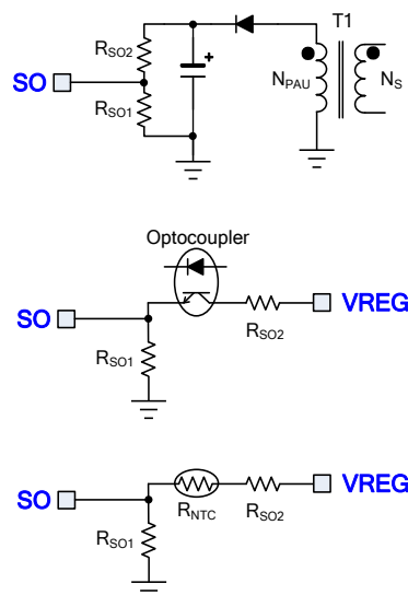
Figure 42: SO Application Circuit for OVP and External TSD
