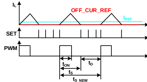
Figure 22: VF-DCM Control Signals
