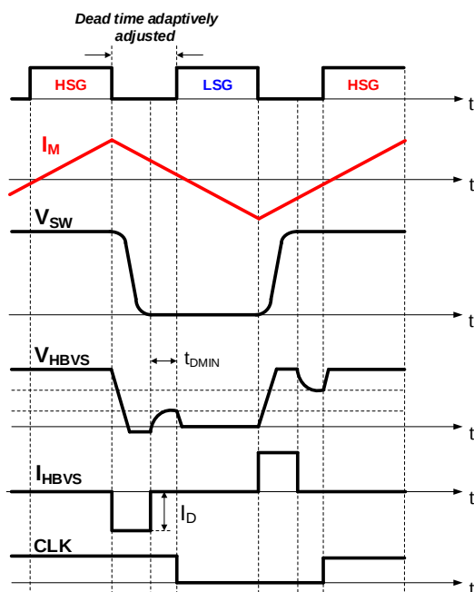
Figure 35: ADTA Operation Waveform
