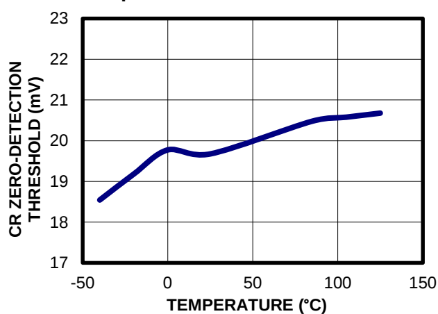
CR Zero-Detection Threshold vs. Temperature
