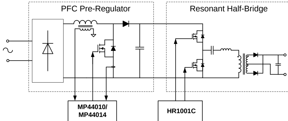
Figure 25: Application Circuit
