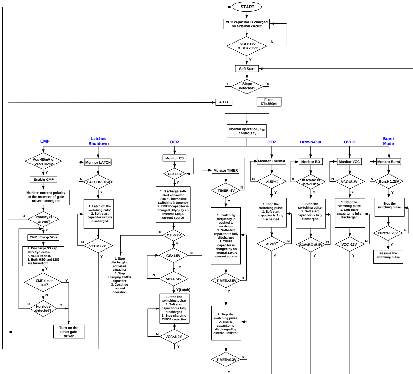
Figure 24: Control Flow Chart
