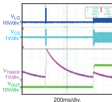
OCP or SCP Recovery
