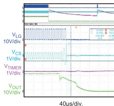
Short Circuit Protection Entry
