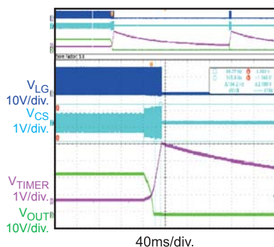
Over-Current Protection Entry
