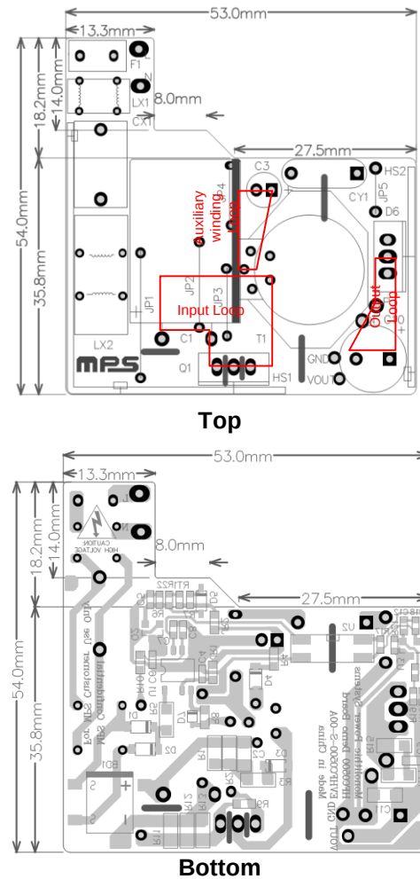
Figure 16: Recommended Layout
