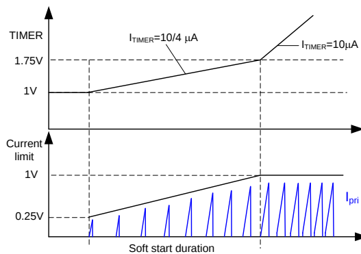
Figure 6: Soft Start
