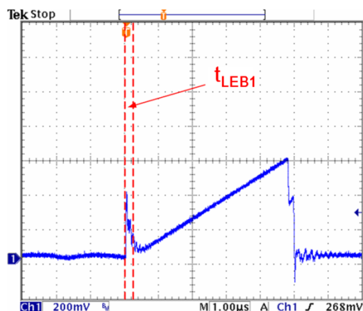
Figure 5: Leading-Edge Blanking
