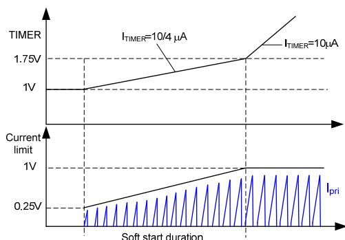
Figure 6: Soft Start
