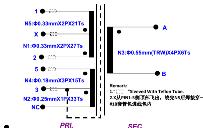
Figure 5: Electrical Diagram
