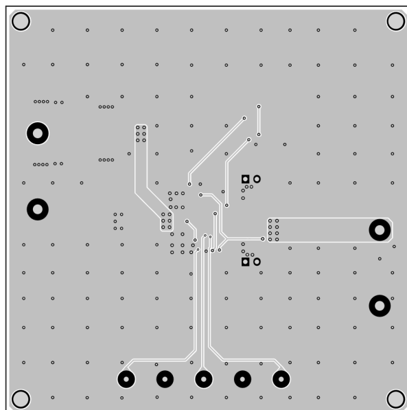
Figure 3: Inner 2 Layer
