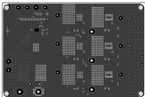
Figure 4: Mid-Layer 1
