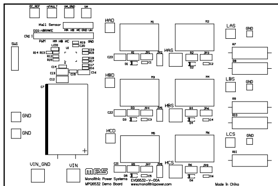
Figure 2: Top Silk
