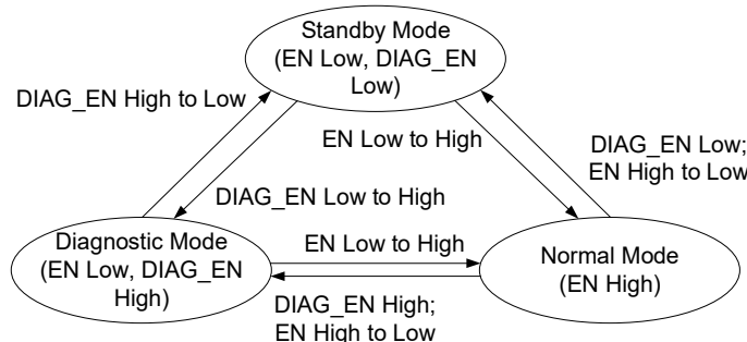
Figure 1: Operation Mode State Machine
