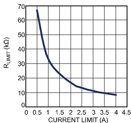
R_{LIMIT} vs. Current Limit
