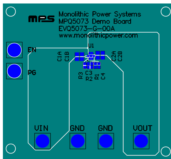
Figure 3: Top Layer
