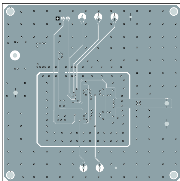
Figure 4: Inner Layer 2
