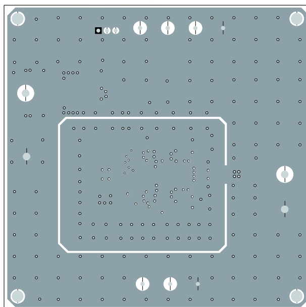
Figure 3: Inner Layer 1
