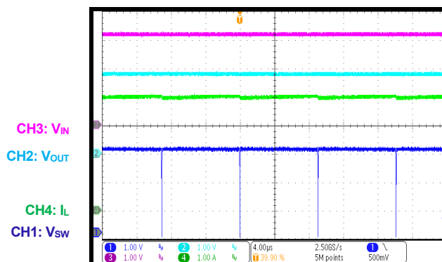
Low-Dropout Mode
