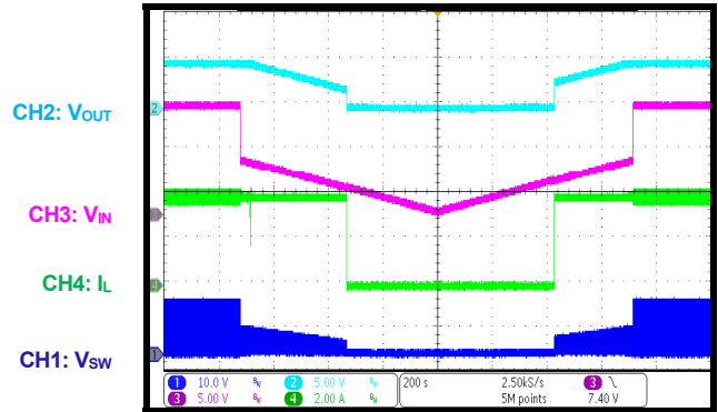
V_{IN} Ramping Down and Up V_{IN} = 6V to 0V , 0.5V/min , I_{OUT} = 4A
