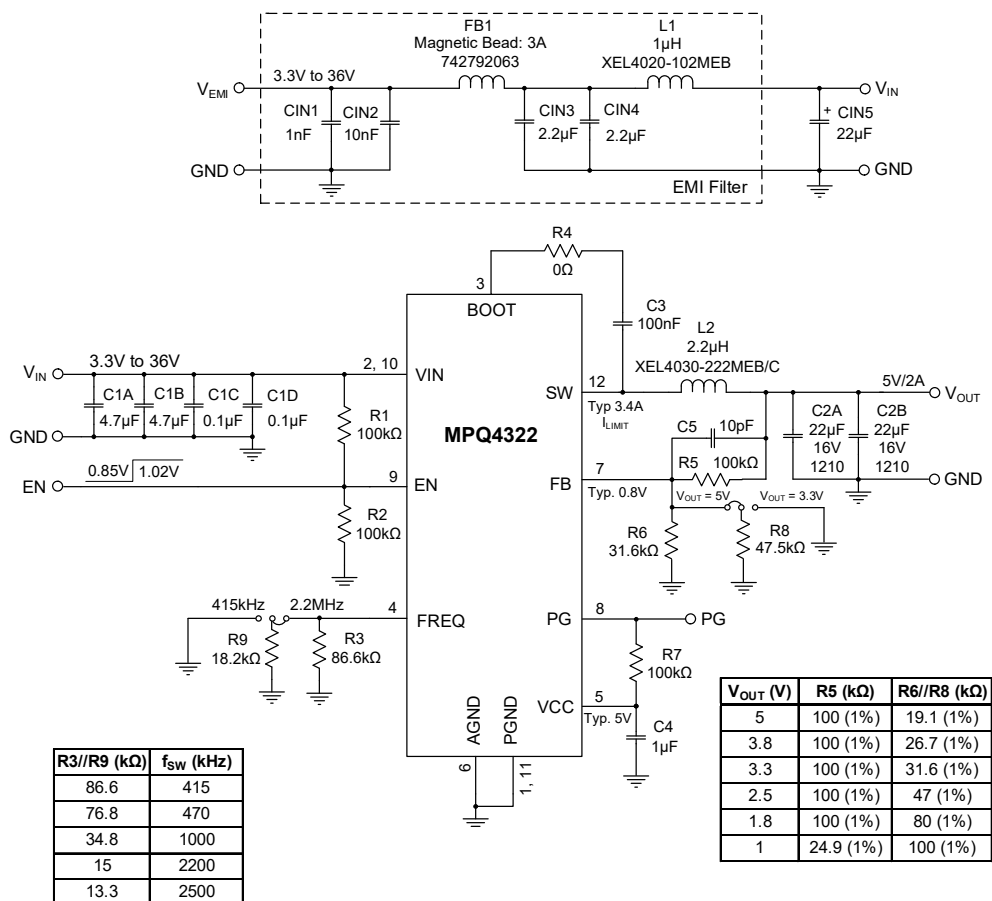
Figure 3: Evaluation Board Schematic
