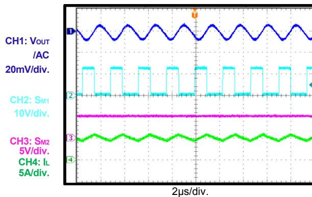
Steady state , V_{OUT}=12V , BB_FSW=1 , Load=5A
