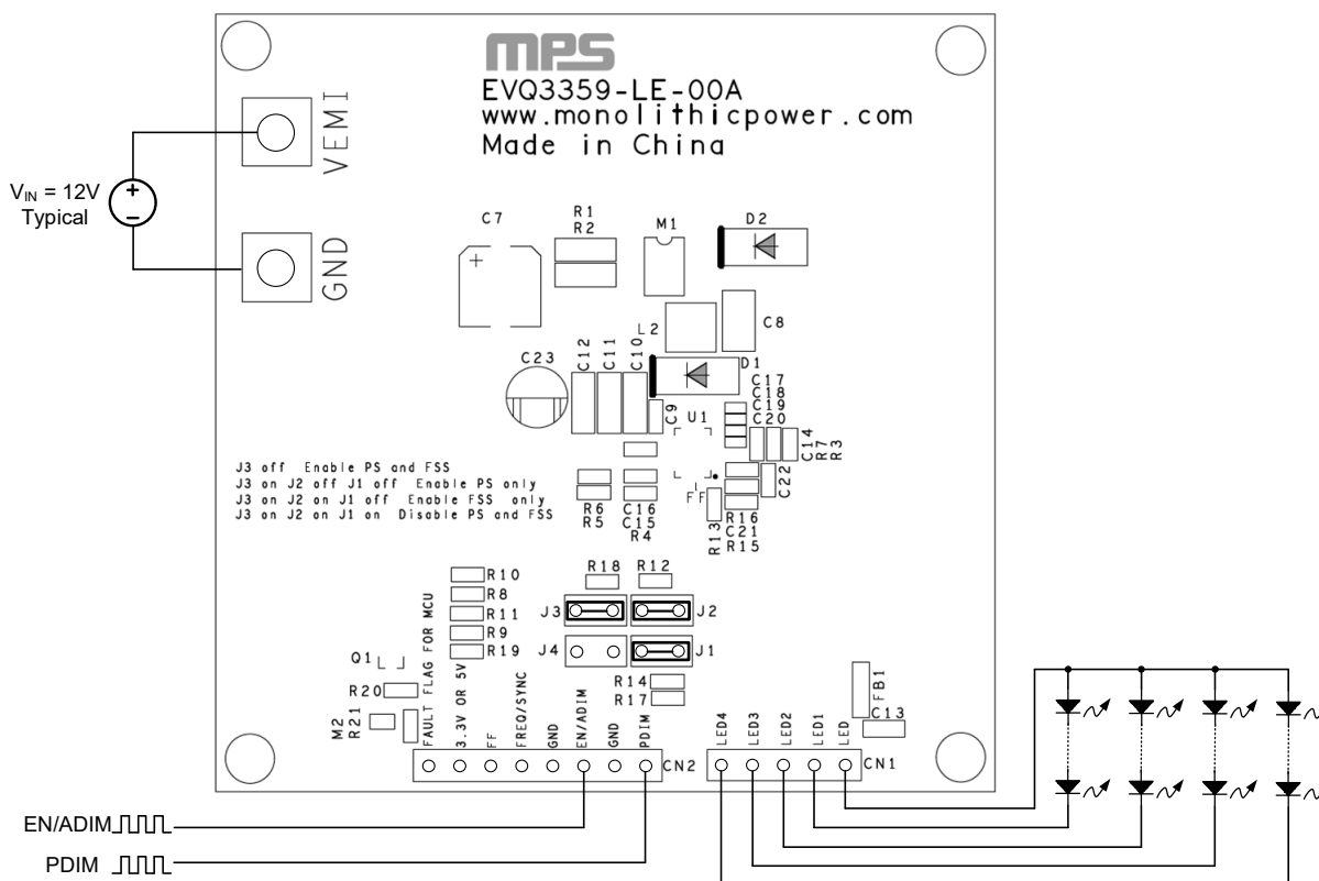
Figure 1: Measurement Equipment Set-Up (1) (2) (3) (4) (5)
