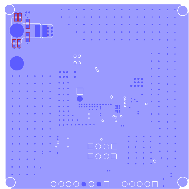
Figure 6: Bottom Layer
