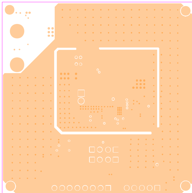
Figure 4: Mid-Layer 1
