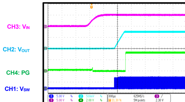
PG Start-Up through VIN
