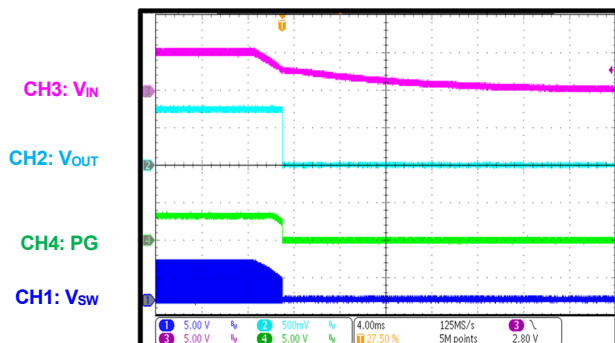
PG Shutdown through VIN
