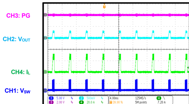
SCP Steady State
