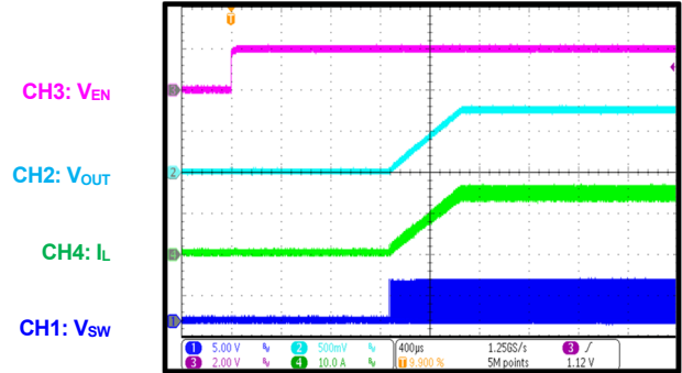
Start-Up through EN I_{OUT} = 14A
