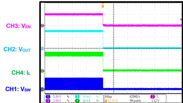
Shutdown through EN I_{OUT} = 14A
