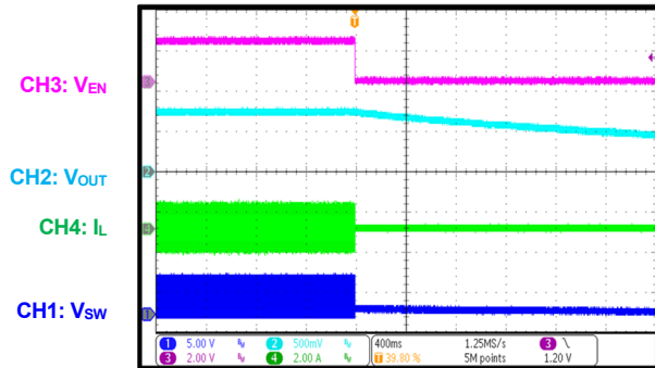
Shutdown through EN I_{OUT} = 0A , FCCM
