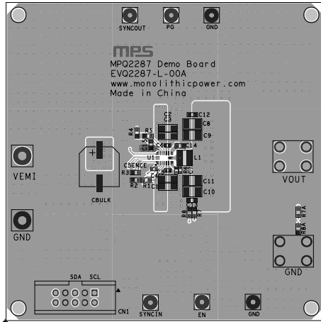
Figure 4: Top Silk and Top Layer
