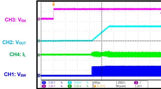
Start-Up through EN I_{OUT} = 0A , FCCM
