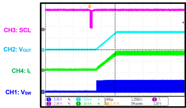
Start-Up via the Digital Interface I_{OUT} = 14A
