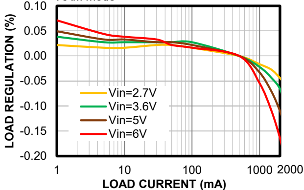
Load Regulation
