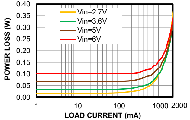
Power Loss vs. Load Current
