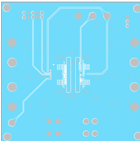
Figure 6: Mid-Layer 2
