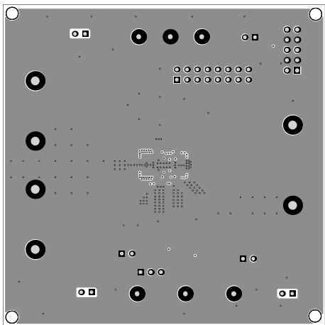
Figure 5: Mid-Layer 1
