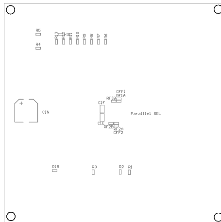
Figure 8: Bottom Silk
