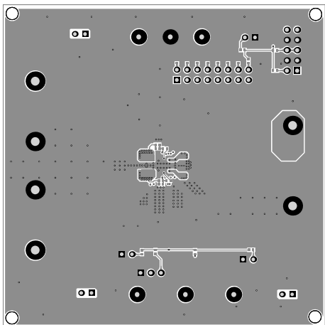
Figure 7: Bottom Layer
