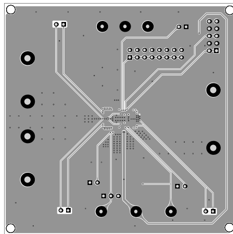
Figure 6: Mid-Layer 2
