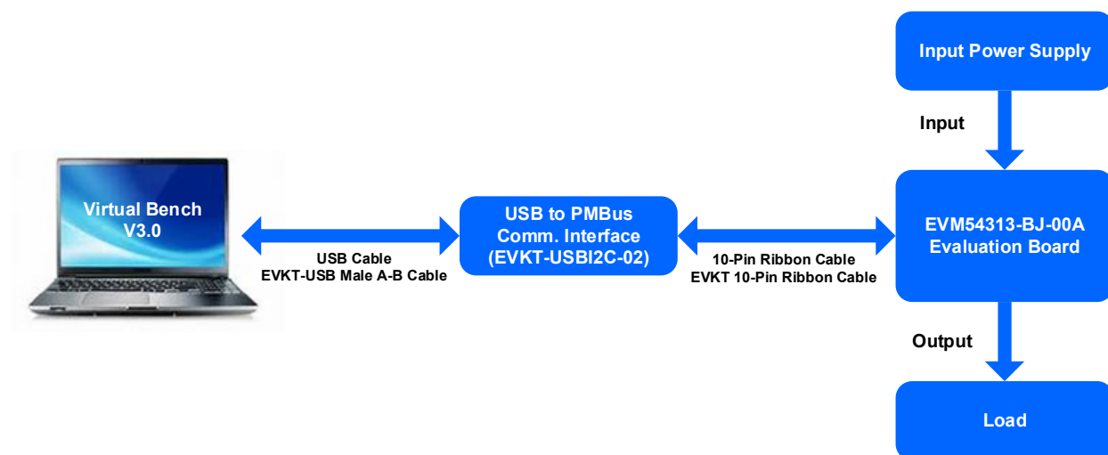
Figure 2: Hardware Set-Up
