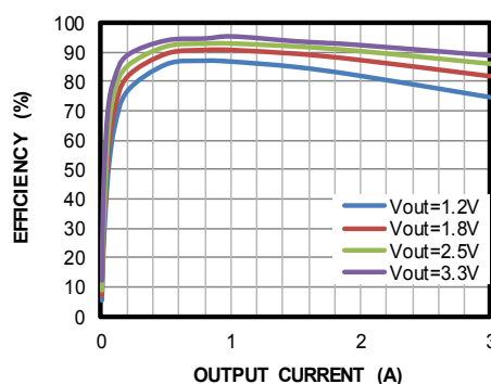
Efficiency vs. Output Current V_{IN}=5V
