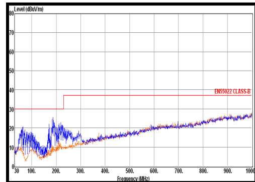
Radiated Emission
