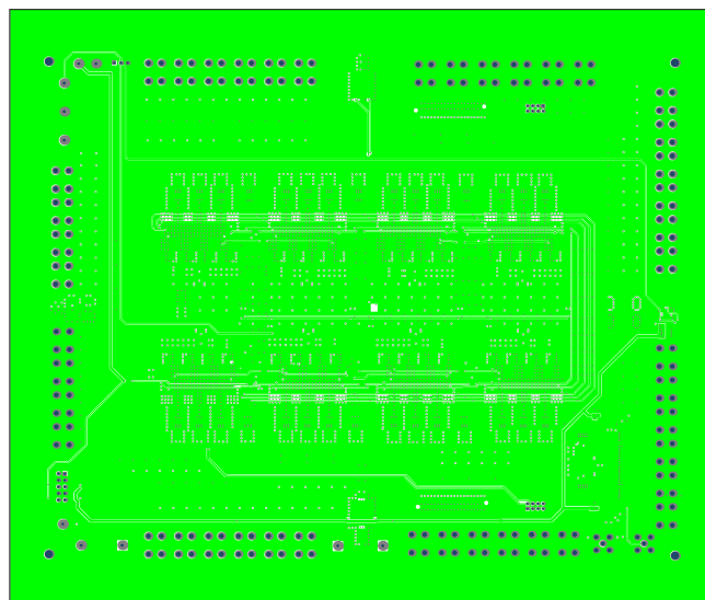
Figure 25: Mid-Layer 4
