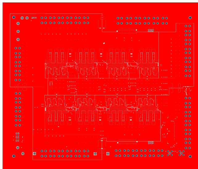
Figure 21: Top Layer
