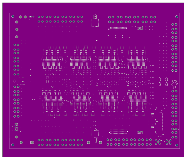
Figure 23: Mid-Layer 2
