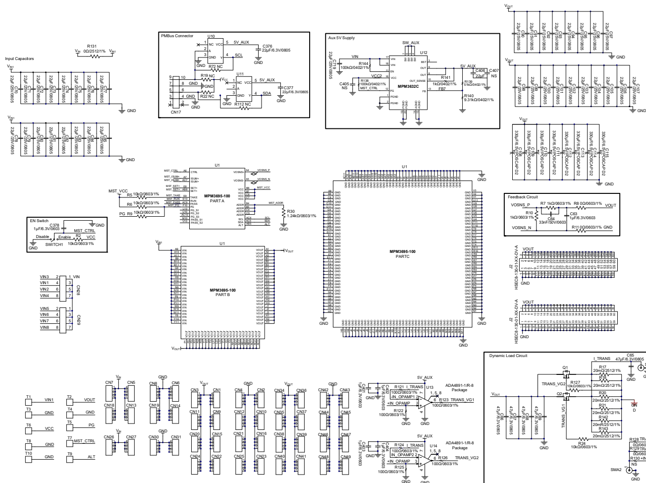
Figure 12: Evaluation Board Schematic (Part 2)
