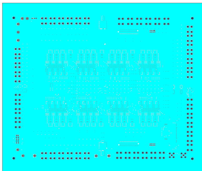
Figure 26: Mid-Layer 5
