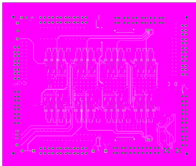
Figure 24: Mid-Layer 3
