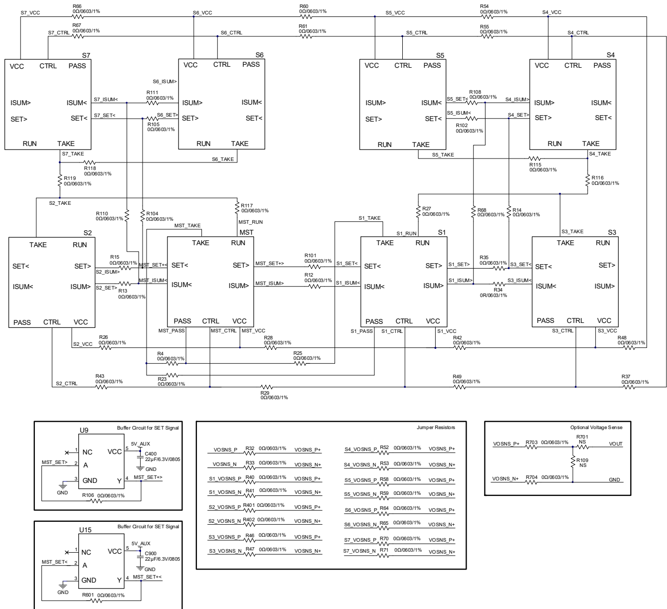
Figure 11: Evaluation Board Schematic (Part 1)
