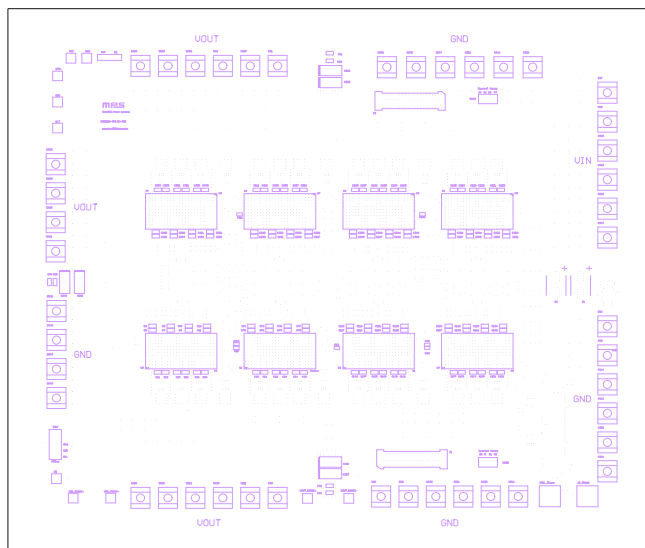
Figure 20: Top Silk
