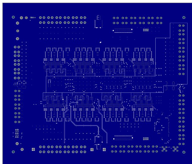
Figure 27: Mid-Layer 6
