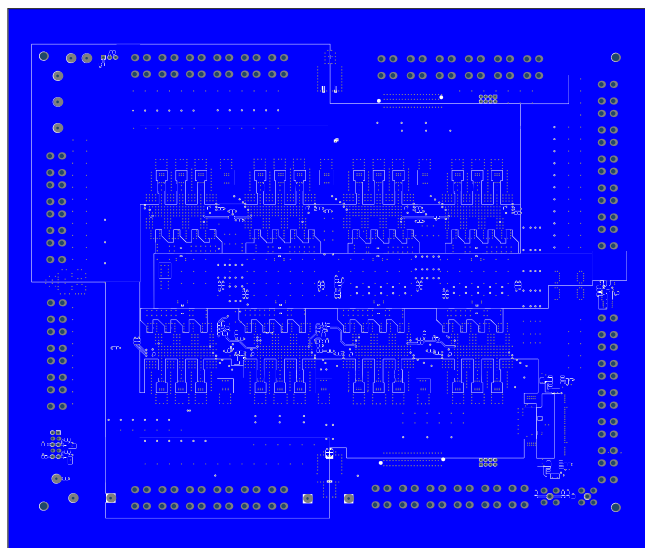
Figure 28: Bottom Layer
