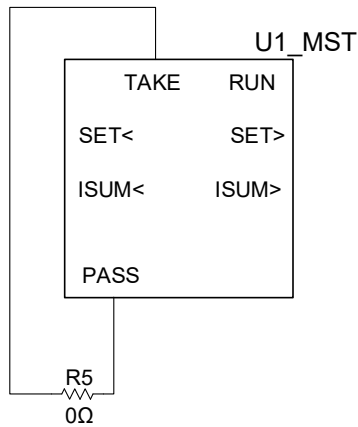
Figure 11: EVM3695-100-BH-00A Connection Diagram
