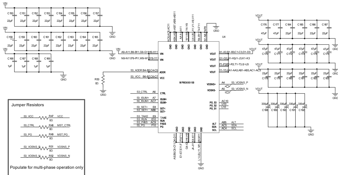
Figure 17: Schematic of Slave 3
