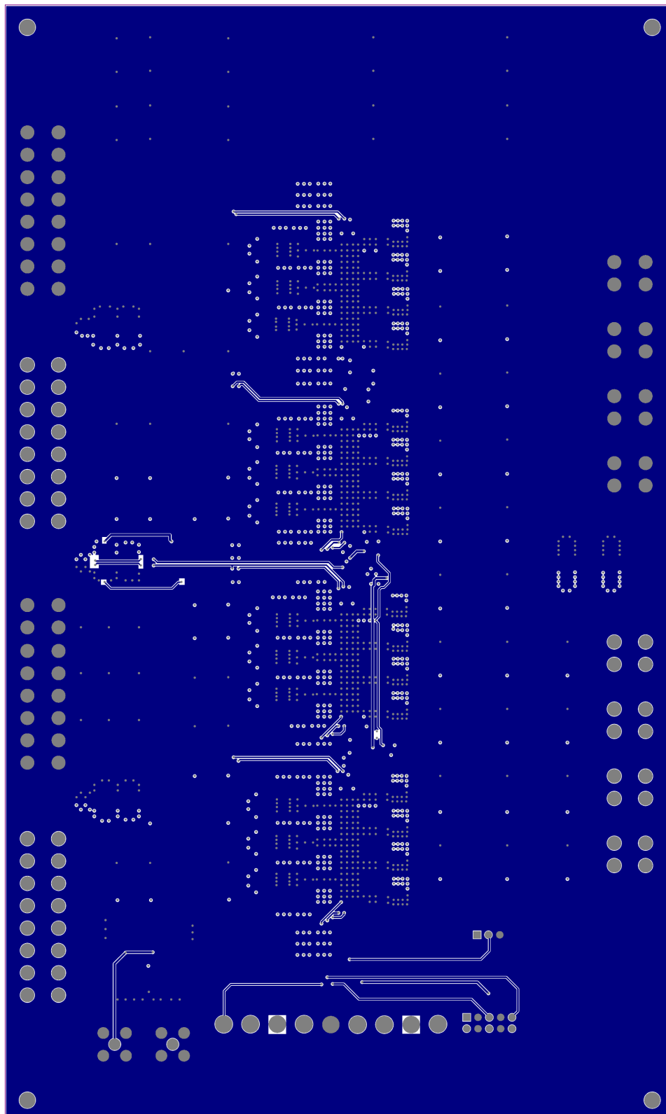
Figure 22: Mid-Layer 3
