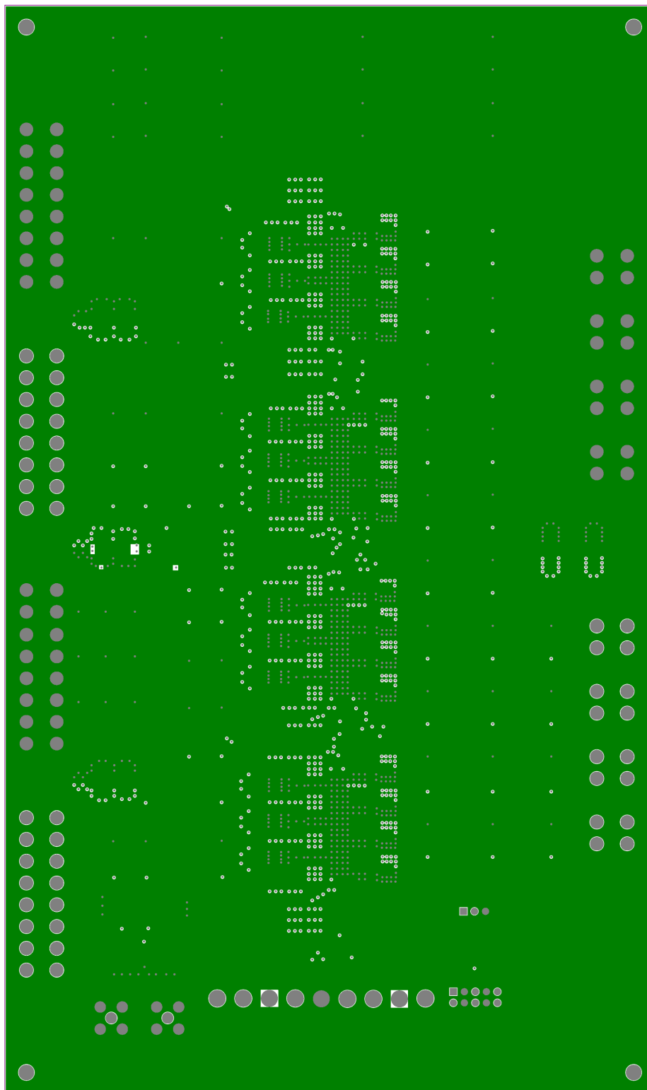
Figure 20: Mid-Layer 1
