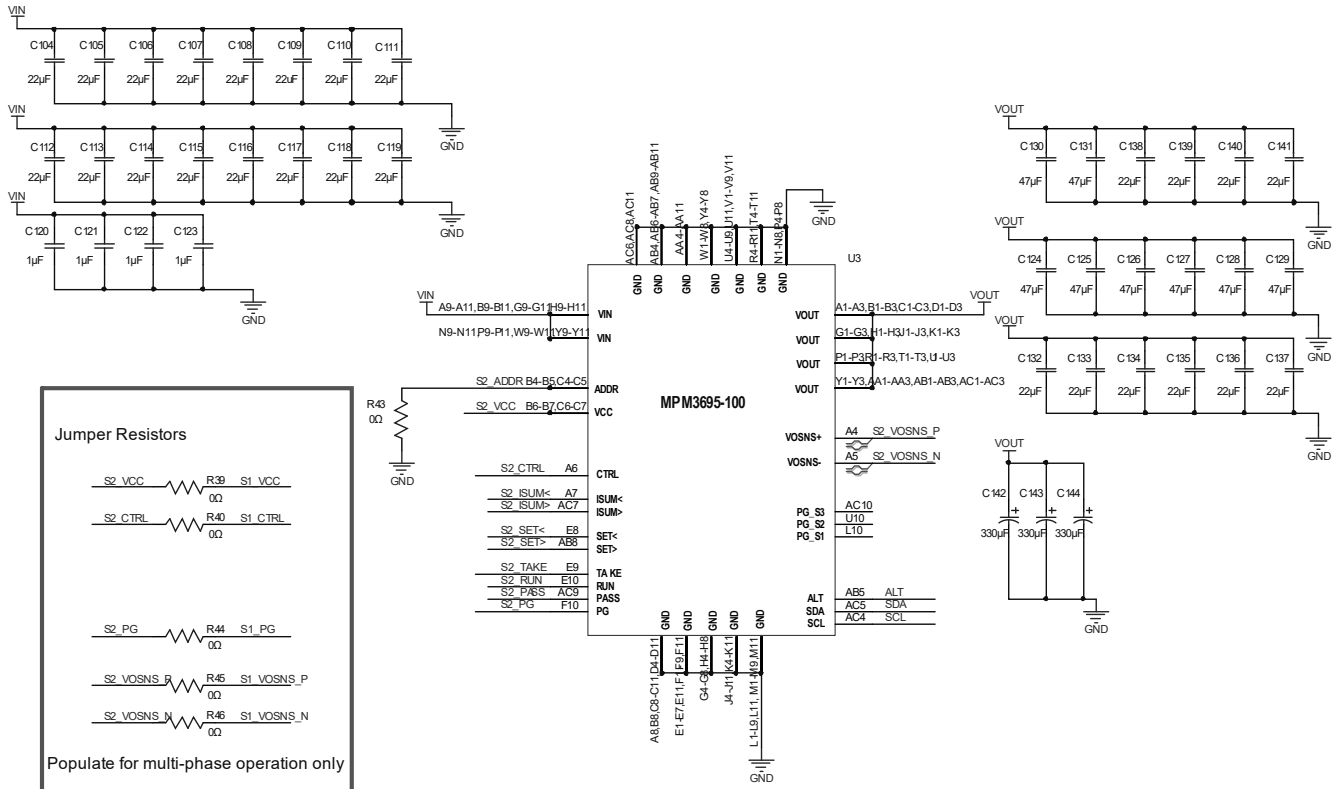
Figure 16: Schematic of Slave 2
