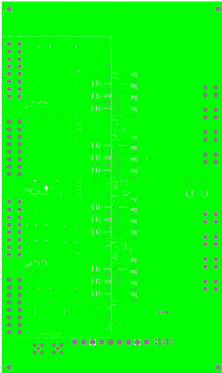
Figure 21: Mid-Layer 2
