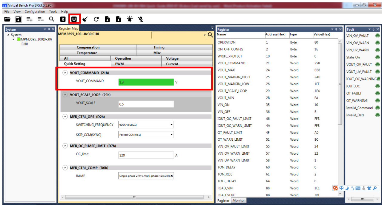
Figure 7: Writing Values to the Register
