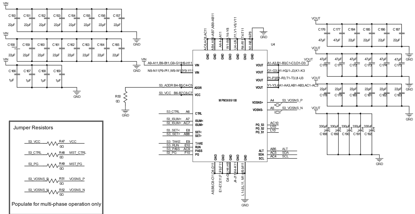
Figure 17: Schematic of Slave 3
