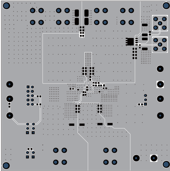
Figure 13: Bottom Layer
