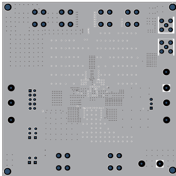
Figure 11: Mid-Layer 1
