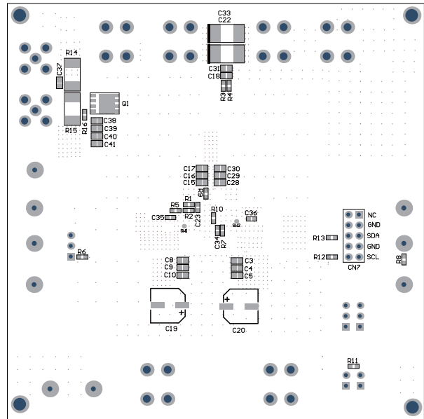
Figure 14: Bottom Silk
