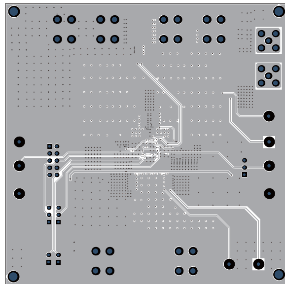
Figure 12: Mid-Layer 2
