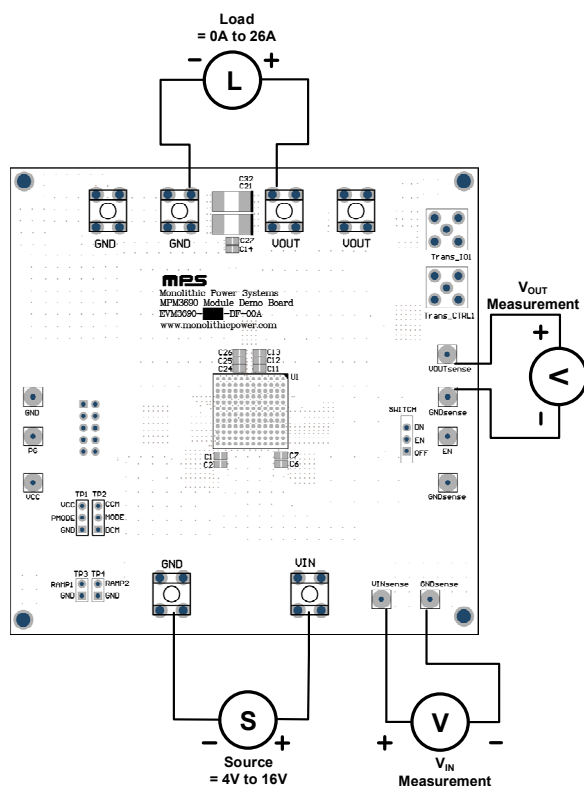
Figure 1: Proper Measurement Equipment Set-Up
