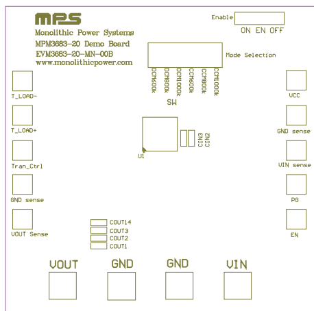
Figure 3: Top Silk
