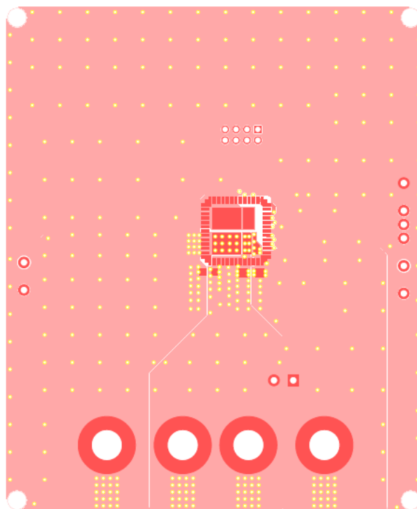
Figure 2: Top Layer
