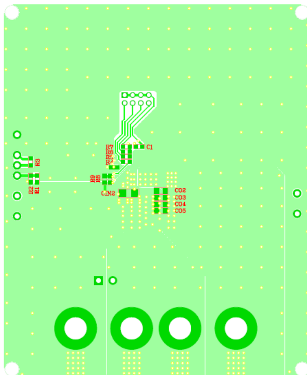
Figure 4: Bottom Layer
