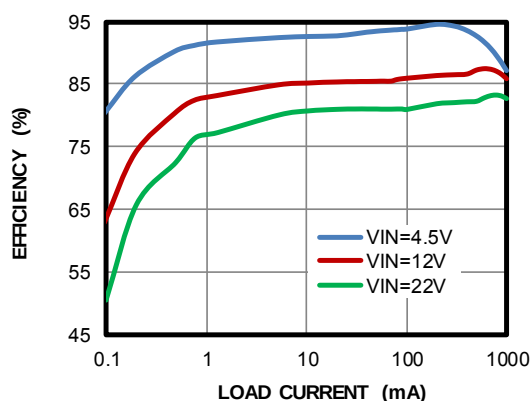
Efficiency vs. Load Current V OUT = 3.3V
