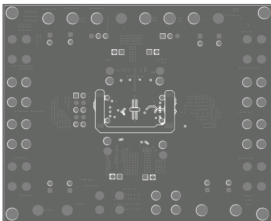
Figure 5: Mid-Layer 1
