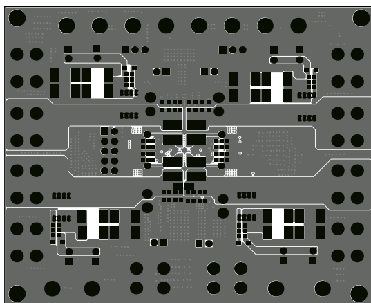
Figure 7: Bottom Layer
