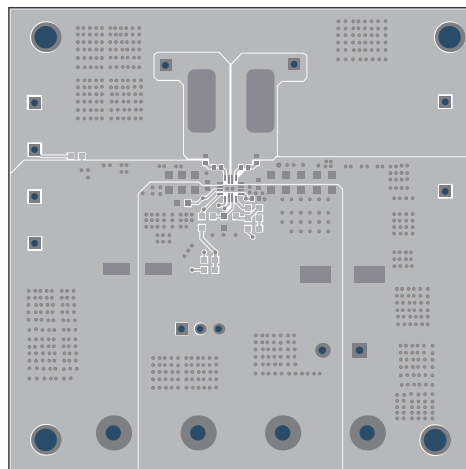
Figure 3: Top Layer
