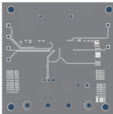
Figure 5: Mid-Layer 2
