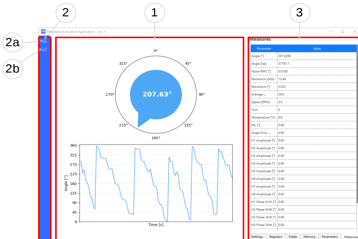
Figure 15: Application Layout
