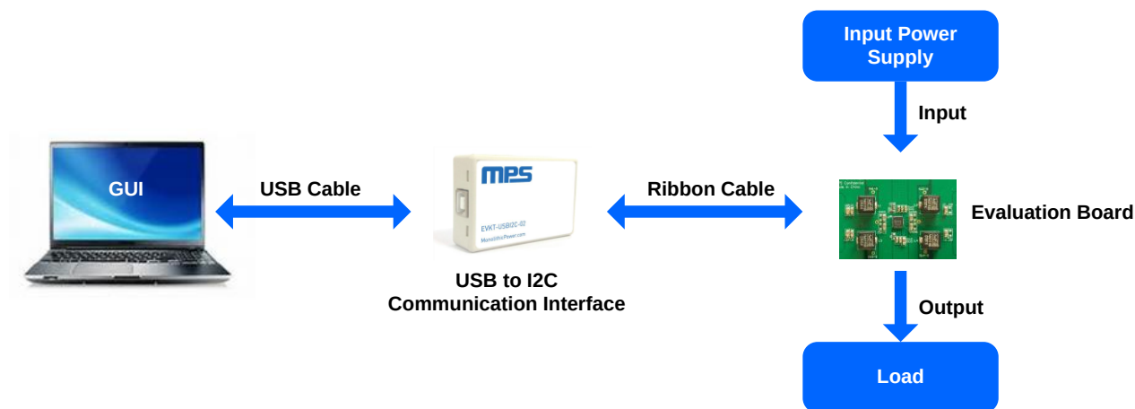
Figure 1: EVKT-MP5470 Evaluation Kit Set-Up
