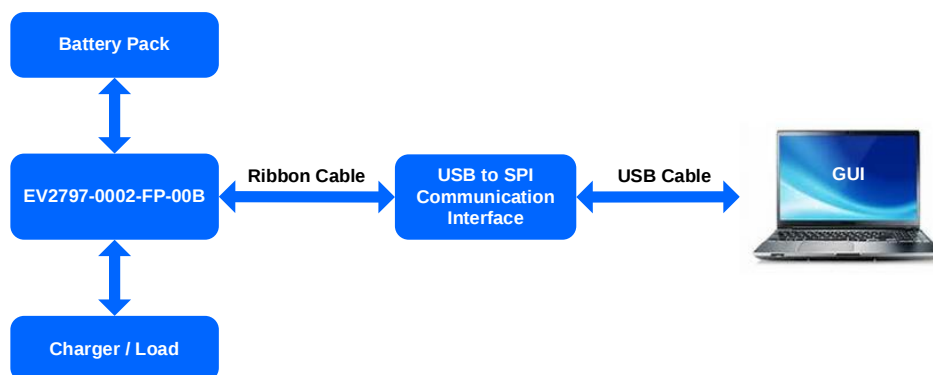
Figure 2: EVKT- MP2797-0002 Evaluation Kit Set-Up
