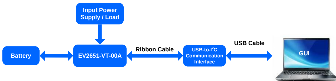
Figure 1: EVKT-MP2651 Evaluation Kit Set-Up
