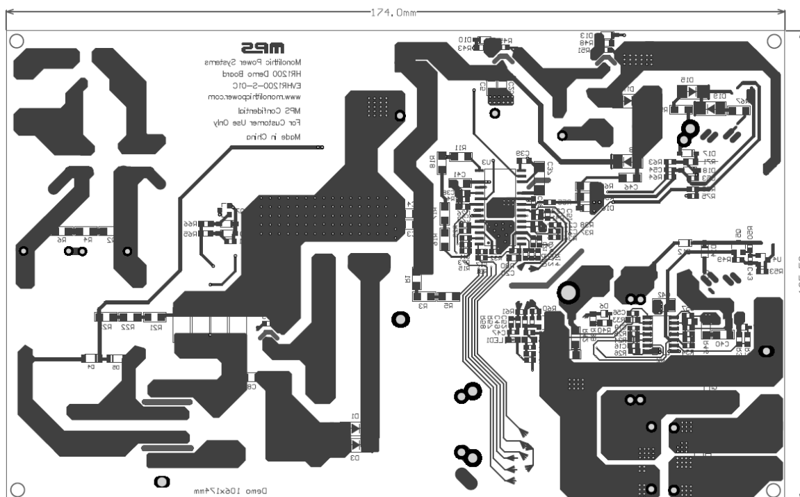
Figure 2: Bottom Layer
