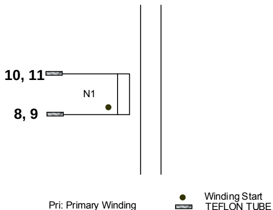
Electrical Diagram
