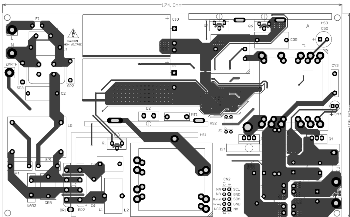
Figure 1: Top Layer
