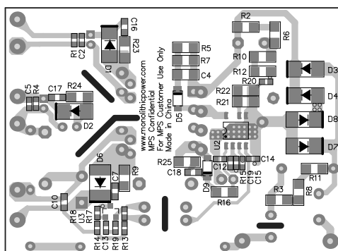
Figure 3: Bottom Layer
