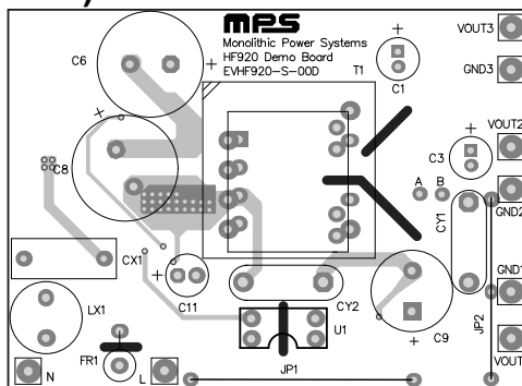
Figure 2:Top Layer
