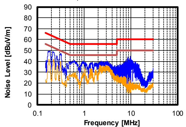
Conducted EMI Two-Wire Input, N Line
